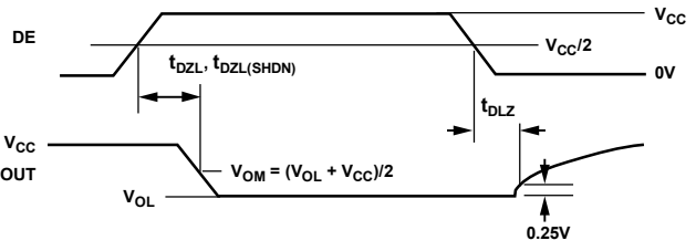
Figure 11. Driver Enable and Disable Times ( t_{DZL} , t_{DLZ} , t_{DZL(SHDN)} )
