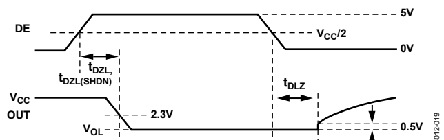
Figure 19. Driver Enable and Disable Times ( t_{DZL} , t_{DZL(SHDN)} , t_{DLZ} , t_{DLZ} )
