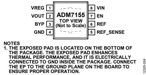
Figure 4. 8-Lead SOIC Pin Configuration
