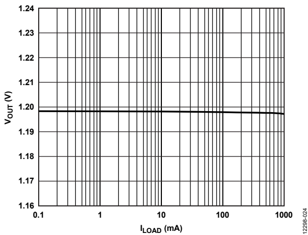
Figure 24. Output Voltage ( V_{OUT} ) vs. Load Current ( I_{LOAD} ), Adjustable Version, V_{OUT} = 1.2V
