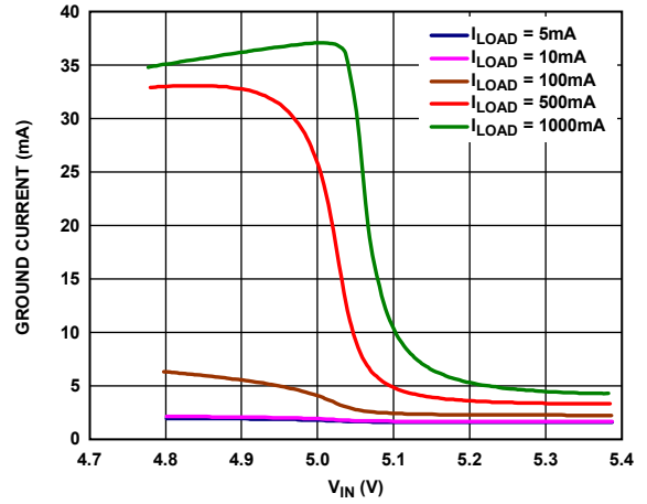
Figure 13. Ground Current vs. Input Voltage (VIN) in Dropout, VOUT = 5 V
