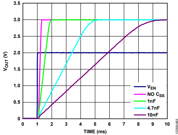
Figure 61. Typical Soft Start Behavior, Different C SS Values
