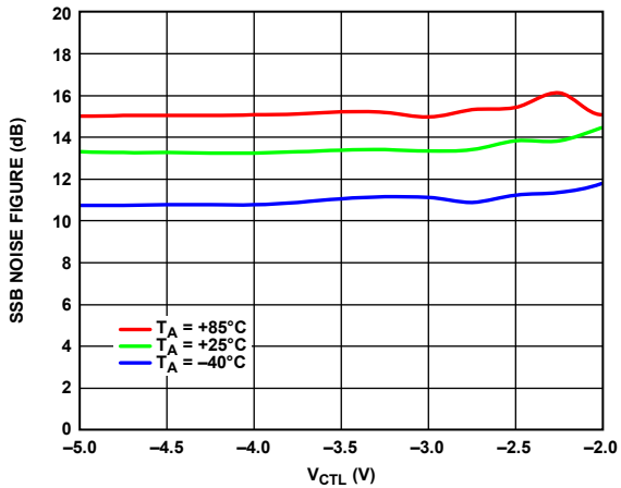
Figure 31. SSB Noise Figure vs. V_{CTL} at Various Temperatures, RF Frequency = 18 GHz, Lower Sideband
