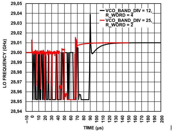
Figure 98. LO Frequency vs. Time, REF_IN Frequency = 200 MHz, f_{BSC} = 4 MHz
