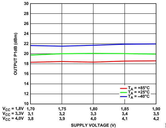
Figure 52. Output P1dB vs. Supply Voltage over Temperature
