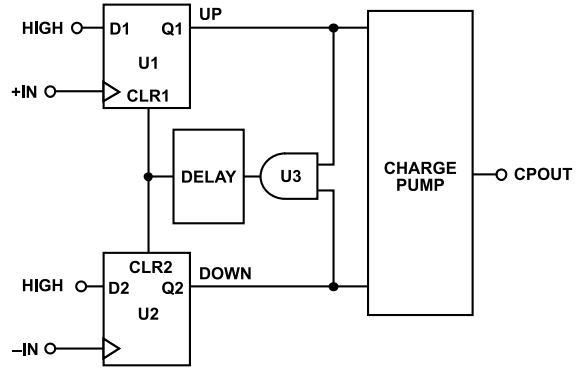
Figure 91. Phase Frequency Detector and Charge Pump Simplified Schematic
