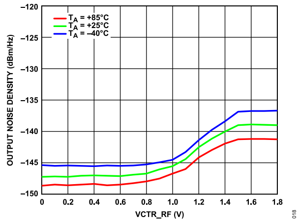
Figure 18. Output Noise Density vs. VCTR RF over Temperature
