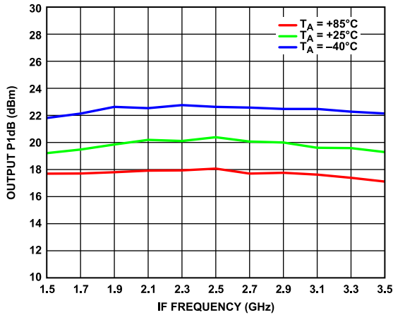
Figure 51. Output P1dB vs. IF Frequency over Temperature
