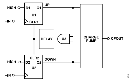
Figure 56. PFD and CP Simplified Schematic
