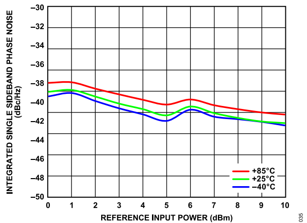
Figure 32. Integrated Single Sideband Phase Noise vs. Reference Input Power over Temperature, 1 kHz to 125 MHz
