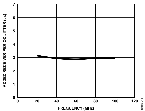
Figure 15. Receiver Jitter (Period) vs. Frequency ( V_{CC} = 3.3 V, T_A = 25 °C, V_{ID} = 400 mV)
