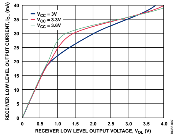
Figure 7. Receiver Output Current vs. Output Voltage (Output Low) ( T_A = 25^\circ\text{C} )
