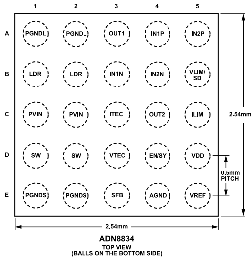
Figure 2. WLCSP Pin Configuration (Top View)
