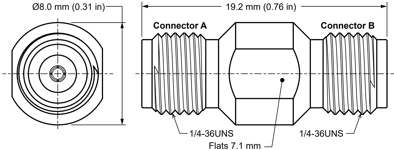
Figure 1: Product Dimensions for the ADP-2.92F-2.92F Adapter
