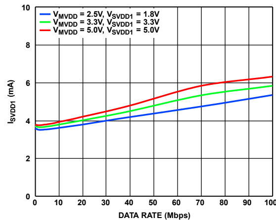
Figure 51. SVDD1 Supply Current ( I_{SVDD1} ) per SPI Input vs. Data Rate at Various Supply Voltages, SSS Is Low, Clock Signal Applied on Single SPI Channel, Other Input Channels Tied Low
