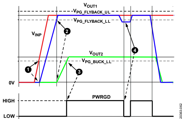
Figure 68. Power Sequencing and PWRGD
