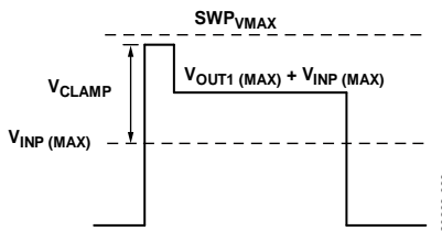
Figure 75. Clamping Waveform
