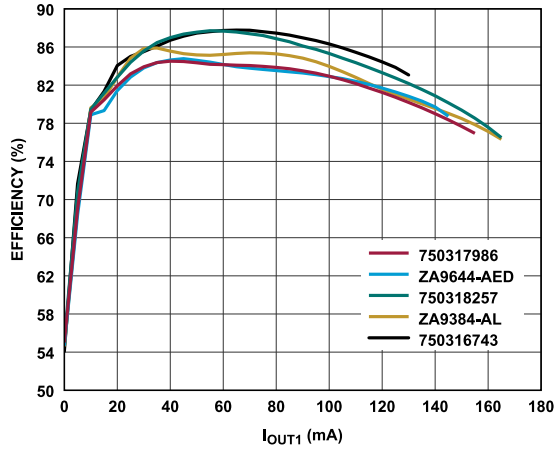
Figure 12. Overall Efficiency Using Various Transformers, T_A = 105^\circ\text{C} , V_{VINP} = 24\text{ V} , V_{OUT1} = 24\text{ V} , V_{OUT2} = 5.0\text{ V} , I_{OUT2} = 6\text{ mA} , V_{OUT3} = -15\text{ V} , I_{OUT3} = -4\text{ mA}
