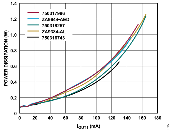
Figure 15. Power Dissipation Using Various Transformers, T_A = 105^\circ\text{C} , V_{VINP} = 24\text{ V} , V_{OUT1} = 24\text{ V} , V_{OUT2} = 5.0\text{ V} , I_{OUT2} = 6\text{ mA} , V_{OUT3} = -15\text{ V} , I_{OUT3} = -4\text{ mA}
