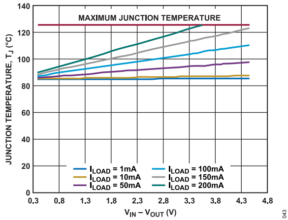
Figure 57. WLCSP, T A = 85°C
