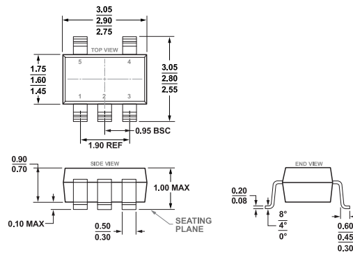
Figure 63. 5-Lead Thin Small Outline Transistor Package [TSOT] (UJ-5) Dimensions shown in millimeters
