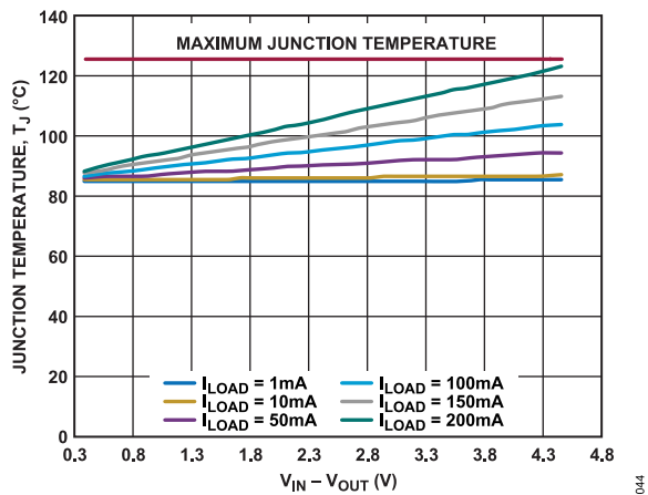
Figure 58. TSOT, T A = 85°C
