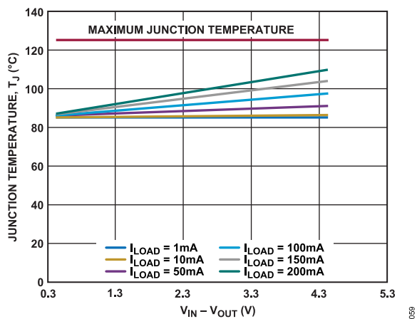
Figure 59. LFCSP, T A = 85°C
