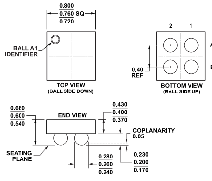
Figure 64. 4-Ball Wafer Level Chip Scale Package [WLCSP] (CB-4-3) Dimensions shown in millimeters
