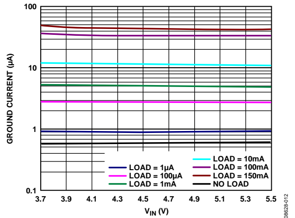
Figure 12. Ground Current vs. Input Voltage ( V_{IN} )
