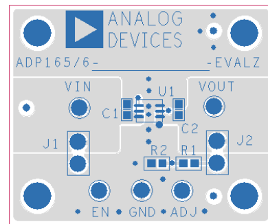
Figure 60. Example of 6-Lead LFCSP PCB Layout
