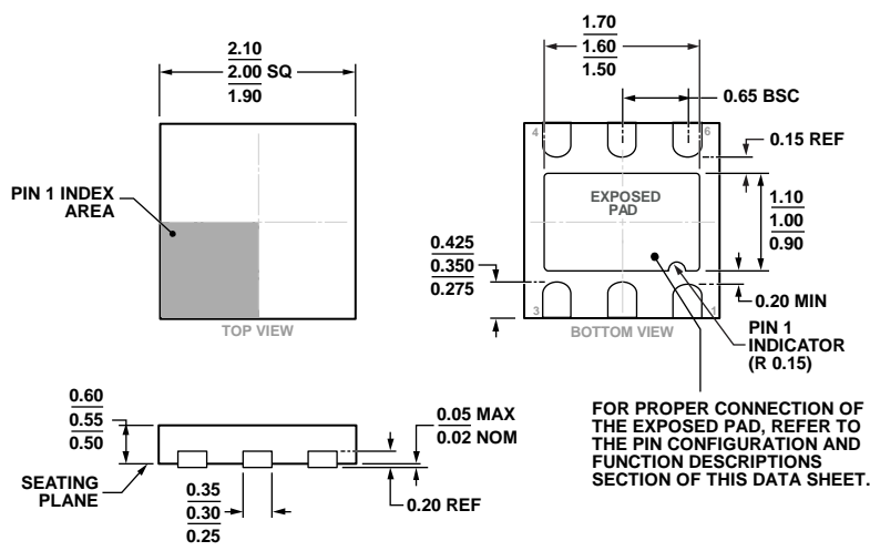
Figure 63. 6-Lead Lead Frame Chip Scale Package [LFCSP_UD] 2.00 mm x 2.00 mm Body, Ultra Thin, Dual Lead (CP-6-3) Dimensions show in millimeters
