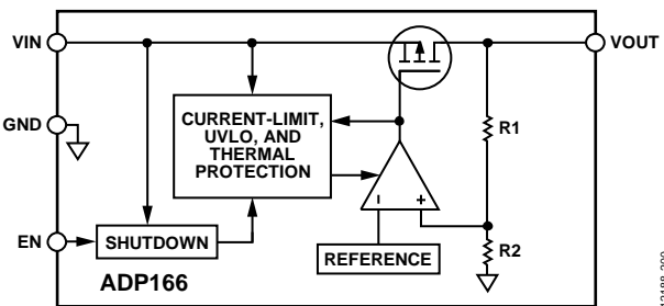
Figure 34. Internal Block Diagram, Fixed Output Without Output Discharge Function
