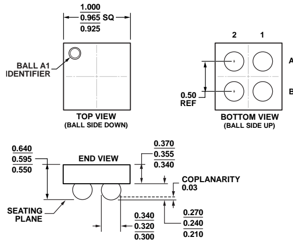
Figure 62. 4-Ball Wafer Level Chip Scale Package [WLCSP] (CB-4-1) Dimensions shown in millimeters
