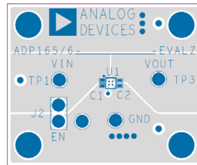
Figure 59. Example of 4-Ball WLCSP PCB Layout
