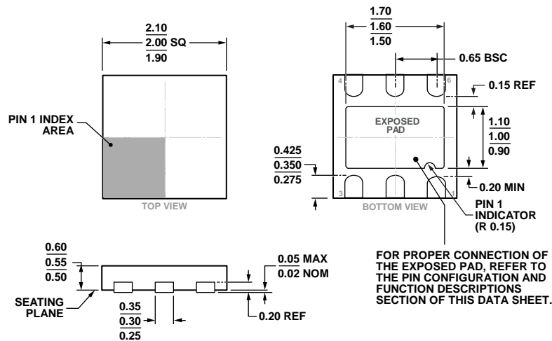
Figure 63. 6-Lead Lead Frame Chip Scale Package [LFCSP_UD] 2.00 mm x 2.00 mm Body, Ultra Thin, Dual Lead (CP-6-3) Dimensions show in millimeters
