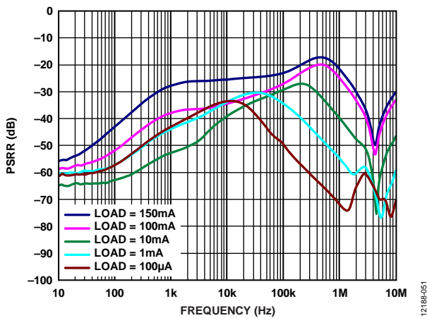
Figure 23. PSRR vs. Frequency, Various Load Currents, V_{OUT} = 2.5 V , V_{IN} = 3.0 V
