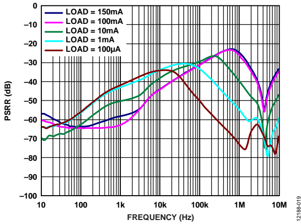
Figure 21. PSRR vs. Frequency, Various Load Currents, V_{OUT} = 3.3 V , V_{IN} = 4.3 V
