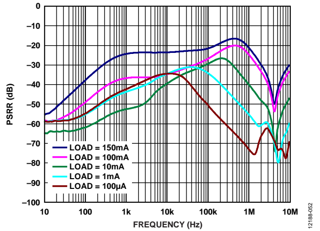
Figure 24. PSRR vs. Frequency, Various Load Currents, V_{OUT} = 3.3 V , V_{IN} = 3.8 V
