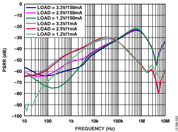
Figure 22. PSRR vs. Frequency, Various Load Currents, V_{IN} - V_{OUT} = 1 V
