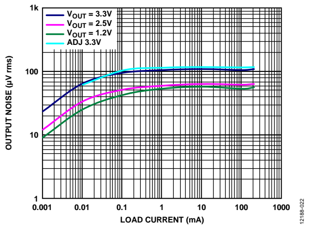
Figure 26. Output Noise vs. Load Current and Output Voltage, V_{IN} = 5 V , C_{OUT} = 1 \mu F
