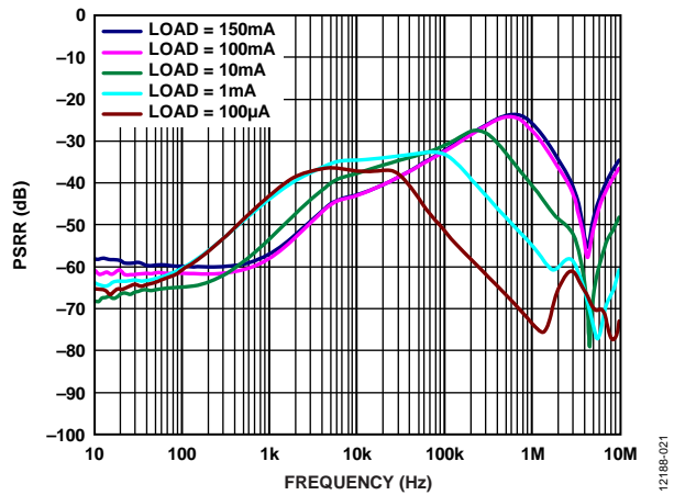
Figure 25. Adjustable ADP165/ADP166 PSRR vs. Frequency, Various Load Currents, V_{OUT} = 3.3 V , V_{IN} = 4.3 V
