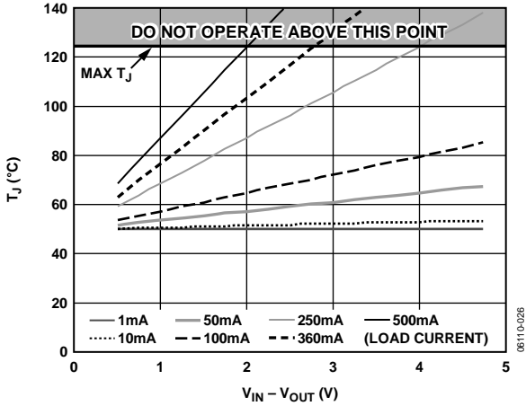
Figure 38. 700 mm 2 of PCB Copper, T A = 50°C
