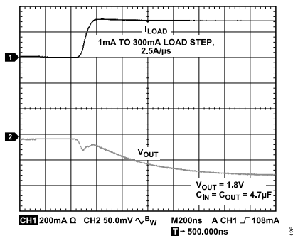
Figure 25. Output Transient Response, C OUT = 4.7 μF
