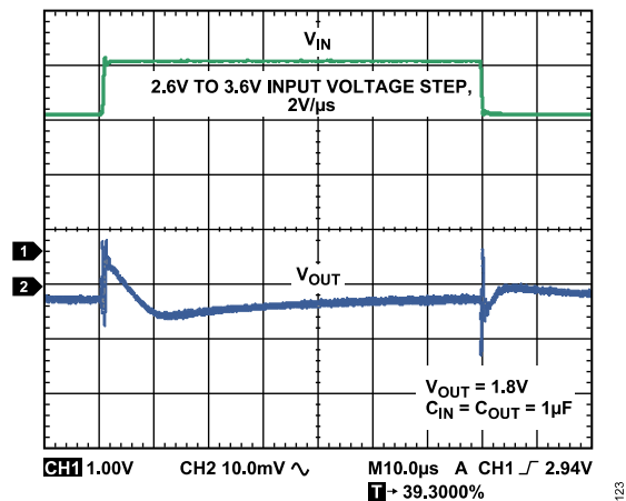
Figure 21. Line Transient Response, Load Current = 1 mA
