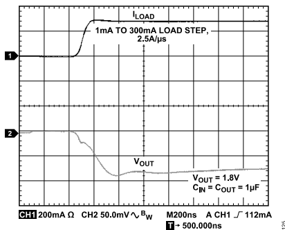
Figure 24. Output Transient Response, C OUT = 1 μF
