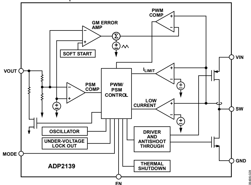
Figure 34. ADP2139 Functional Block Diagram
