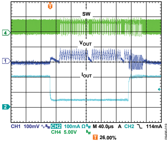
Figure 22. Response to Load Transient, 50 mA to 200 mA, V_{OUT} = 3.3\text{ V} , Automatic Mode
