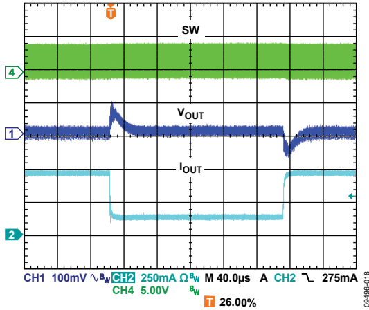
Figure 21. Response to Load Transient, 150 mA to 500 mA, V_{OUT} = 3.3\text{ V} , PWM Mode
