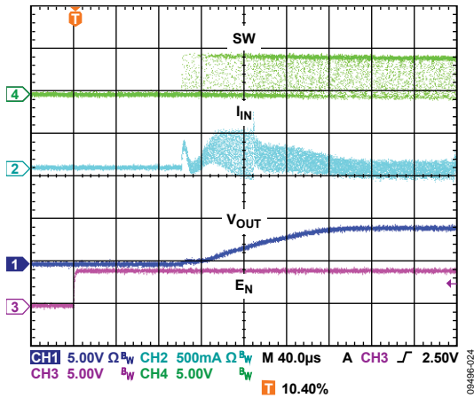
Figure 28. Startup, V_{OUT} = 3.3V , I_{OUT} = 10mA
