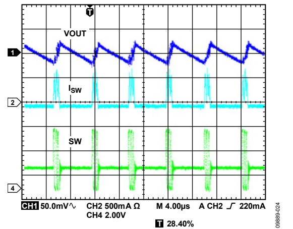
Figure 20. Typical Waveforms, V_{OUT2} = 1.8\text{ V} , I_{OUT2} = 30\text{ mA} , Auto Mode
