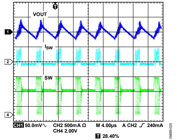
Figure 19. Typical Waveforms, V_{OUT1} = 3.3\text{ V} , I_{OUT1} = 30\text{ mA} , Auto Mode
