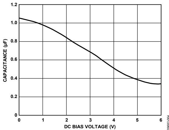
Figure 51. Capacitance vs. Voltage Characteristic
