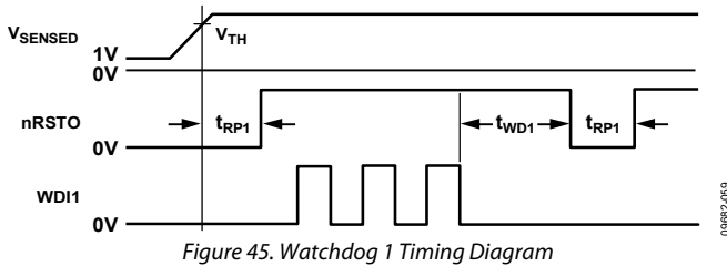
Figure 45. Watchdog 1 Timing Diagram
