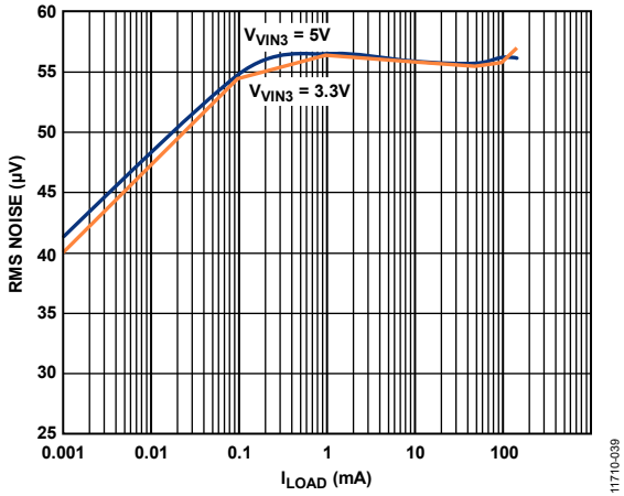
Figure 39. LDO Output Noise vs. Load Current, Across Input Voltage, V_{VIN3} = 5V , V_{VOUT3} = 2.8V
