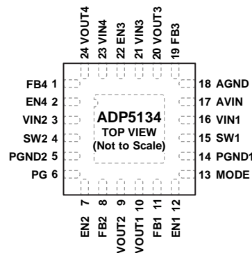
Figure 2. Pin Configuration
