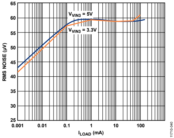
Figure 40. LDO Output Noise vs. Load Current, Across Input Voltage, V_{VIN3} = 5V , V_{VOUT3} = 3.0V
