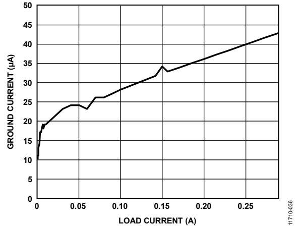
Figure 36. LDO Ground Current vs. Load Current, V_{IN3} = 3.3\text{ V} , V_{OUT3} = 2.8\text{ V}
