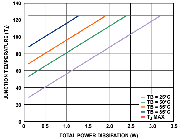
Figure 78. SOIC
