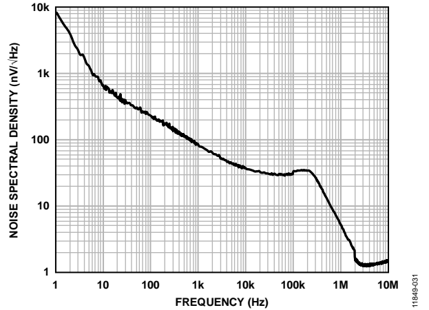
Figure 33. Output Noise Spectral Density vs. Frequency, I_{LOAD} = 10 mA
