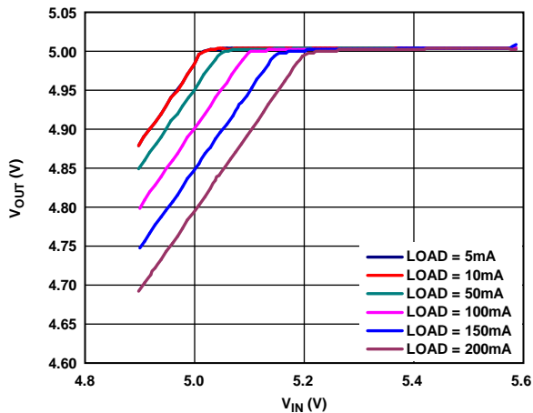
Figure 14. Output Voltage ( V_{OUT} ) vs. Input Voltage ( V_{IN} ) in Dropout, V_{OUT} = 5 V
