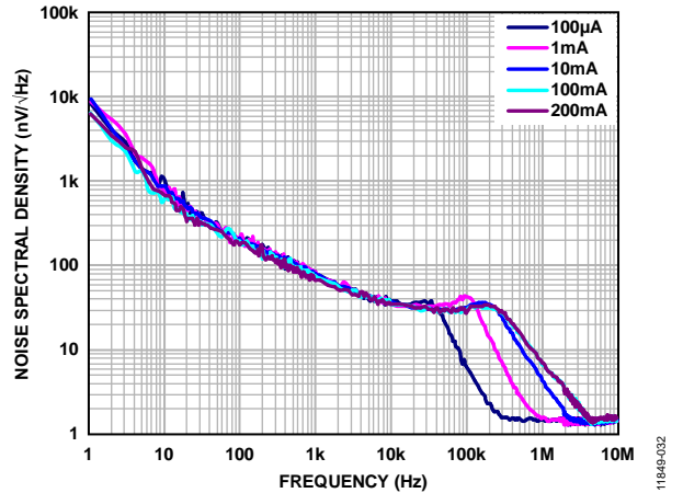
Figure 34. Output Noise Spectral Density vs. Frequency, for Different Loads
