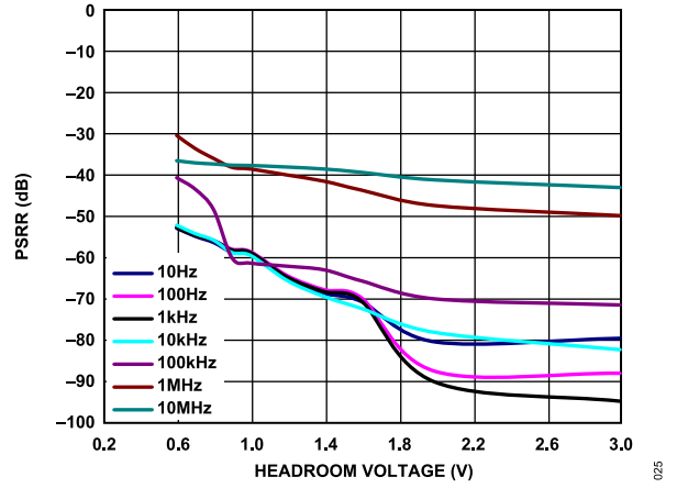
Figure 27. Power Supply Rejection Ratio (PSRR) vs. Headroom Voltage, V_{OUT} = 1.8\text{ V} , for Different Frequencies
