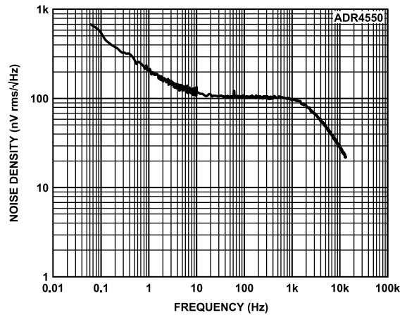
Figure 96. ADR4550 Output Noise Spectral Density
