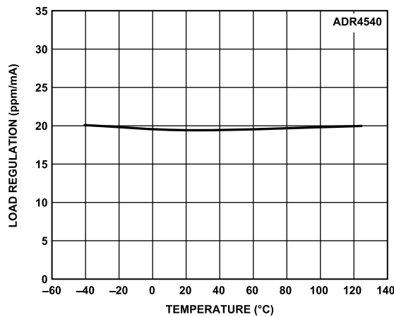
Figure 70. ADR4540 Load Regulation vs. Temperature (Sourcing)
