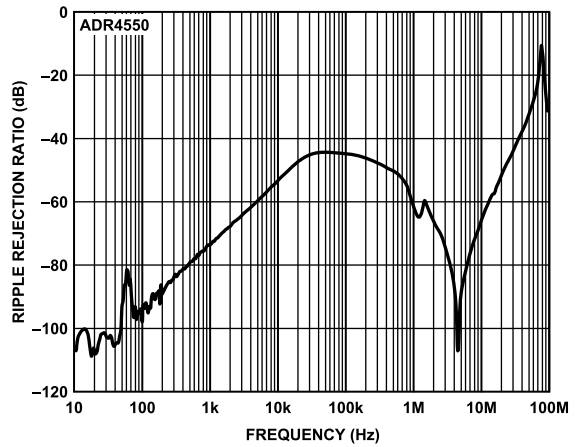
Figure 97. ADR4550 Ripple Rejection Ratio vs. Frequency
