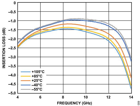
Figure 9. Insertion Loss vs. Frequency over Temperature for RX
