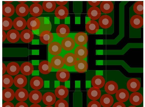
Figure 24. PCB Routings
