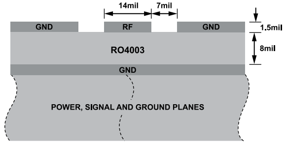
Figure 23. Example PCB Stack-Up
