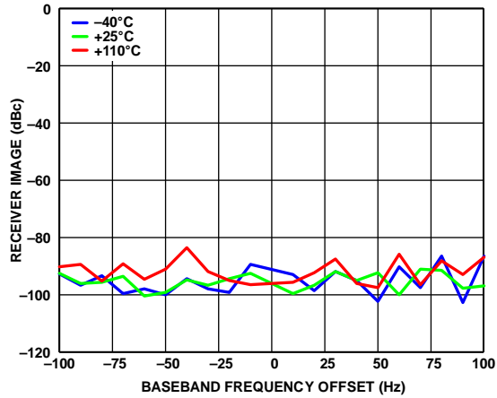
Figure 80. Receiver Image vs. Baseband Frequency Offset, Attenuation = 0 dB, RF Bandwidth = 200 MHz, Tracking Calibration Active, Sample Rate = 245.76 MSPS, LO = 1850 MHz
