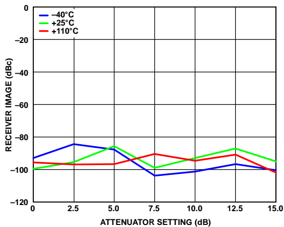
Figure 82. Receiver Image vs. Attenuator Setting, RF Bandwidth = 200 MHz, Tracking Calibration Active, Sample Rate = 245.76 MSPS, LO = 1850 MHz
