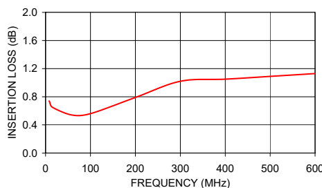
INSERTION LOSS
