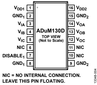
Figure 7. ADuM130D Pin Configuration
