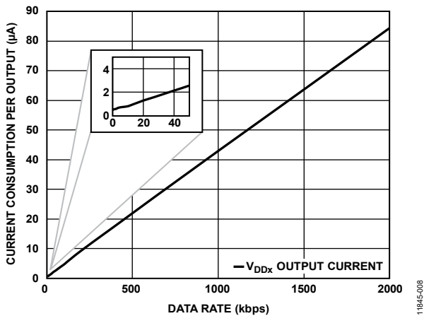
Figure 12. Current Consumption per Output vs. Data Rate for 2.5 V, EN_x = \text{Low Operation}
