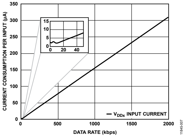
Figure 11. Current Consumption per Input vs. Data Rate for 2.5 V, EN_x = \text{Low Operation}
