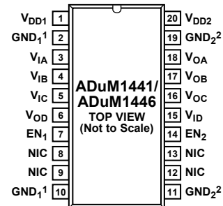
1 PIN 2 AND PIN 10 ARE INTERNALLY CONNECTED. CONNECTING BOTH TO GND 1 IS RECOMMENDED. 2 PIN 11 AND PIN 19 ARE INTERNALLY CONNECTED. CONNECTING BOTH TO GND 2 IS RECOMMENDED.
