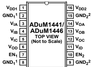
1 PIN 2 AND PIN 8 ARE INTERNALLY CONNECTED. CONNECTING BOTH TO GND 1 IS RECOMMENDED. 2 PIN 9 AND PIN 15 ARE INTERNALLY CONNECTED. CONNECTING BOTH TO GND 2 IS RECOMMENDED.
