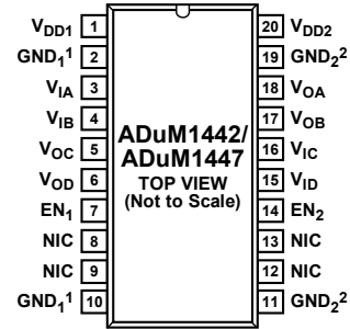
NIC = NOT INTERNALLY CONNECTED.
