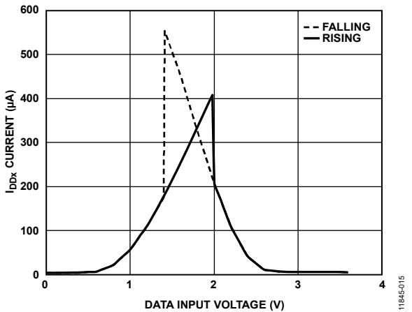
Figure 19. Typical I_{DDx} Current per Input vs. Data Input Voltage for V_{DDx} = 3.3\text{ V}
