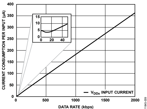
Figure 13. Current Consumption per Input vs. Data Rate for 3.3 V, EN_x = \text{Low Operation}
