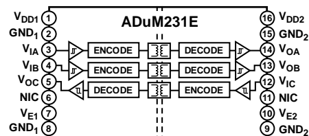
NIC = NO INTERNAL CONNECTION. LEAVE THIS PIN FLOATING. 13577-102
