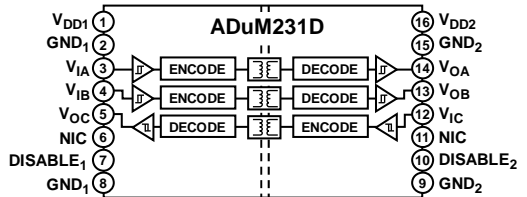
NIC = NO INTERNAL CONNECTION. LEAVE THIS PIN FLOATING. 13577-001
