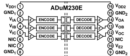
NIC = NO INTERNAL CONNECTION. LEAVE THIS PIN FLOATING. 13577-002
