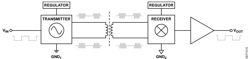
Figure 17. Operational Block Diagram of a Single Channel with a High Fail-Safe Output State
