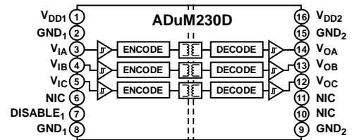
NIC = NO INTERNAL CONNECTION. LEAVE THIS PIN FLOATING. 13577-001
