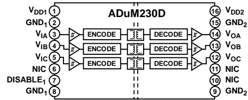
Figure 1. ADuM230D Functional Block Diagram
