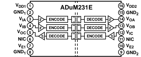
Figure 4. ADuM231E Functional Block Diagram
