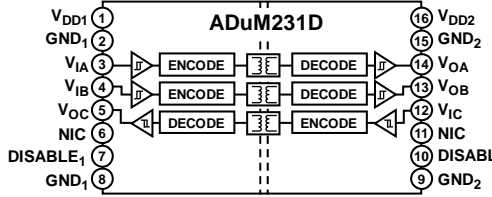
Figure 3. ADuM231D Functional Block Diagram
