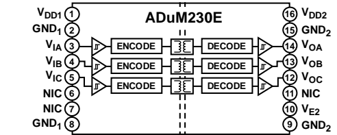
Figure 2. ADuM230E Functional Block Diagram
