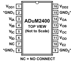
Figure 5. ADuM2400 Pin Configuration
