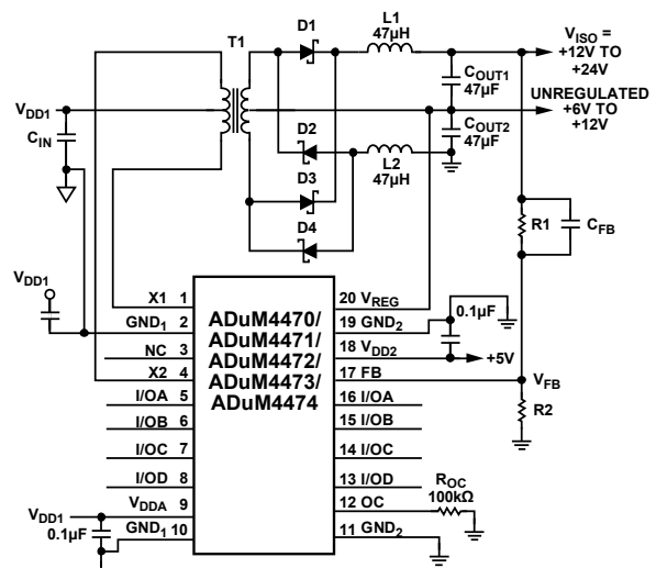
Figure 49. Doubling Power Supply
