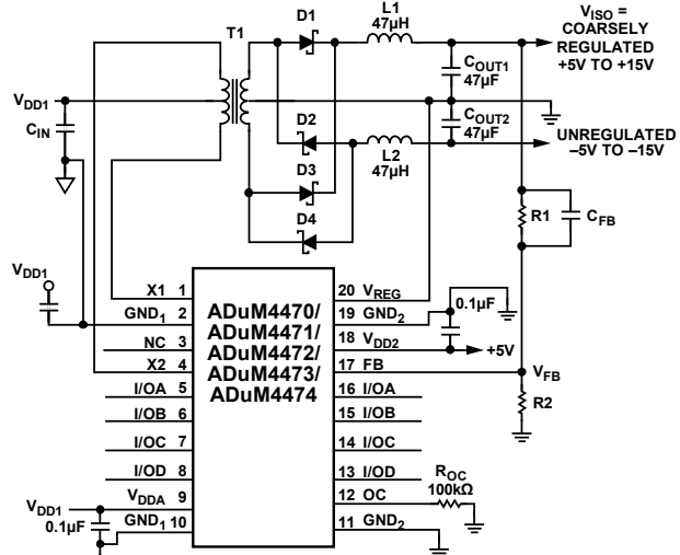
Figure 50. Positive and Unregulated Negative Supply
