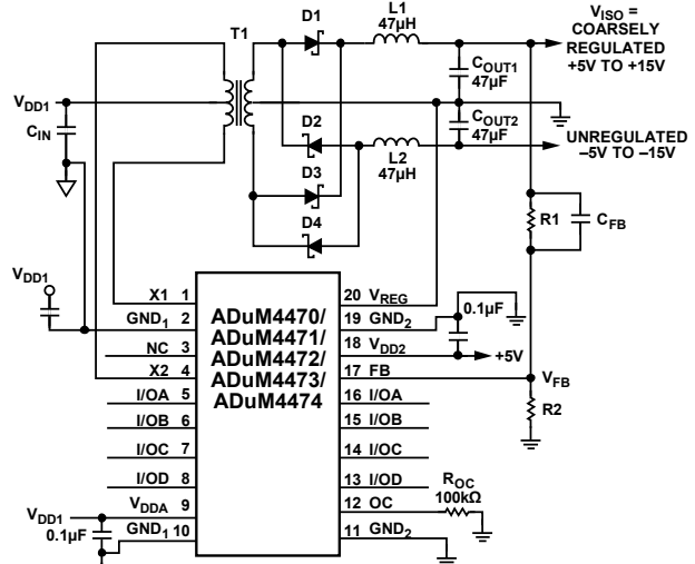
V_{ISO} = V_{FB} \times (R1 + R2)/R2 Figure 50. Positive and Unregulated Negative Supply
