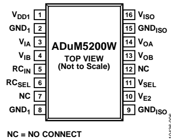
Figure 6. ADuM5200W Pin Configuration
