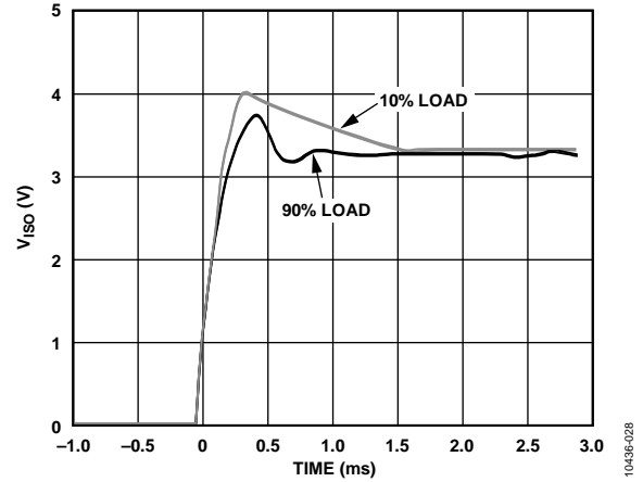
Figure 18. Typical V_{ISO} = 3.3\text{ V} , Output Voltage Startup Transient at 10% and 90% Load
