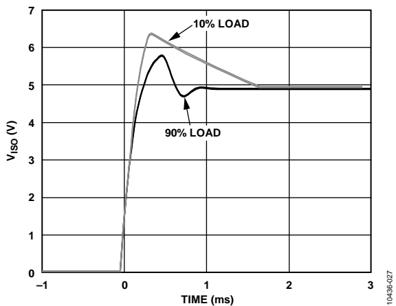
Figure 17. Typical V_{ISO} = 5\text{ V} , Output Voltage Startup Transient at 10% and 90% Load
