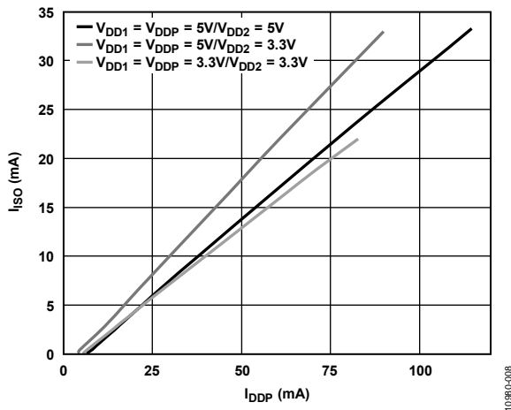
Figure 8. Typical Isolated Output Supply Current, I_{iso} , as a Function of External Load, at 5 V/5 V, 5 V/3.3 V, and 3.3 V/3.3 V
