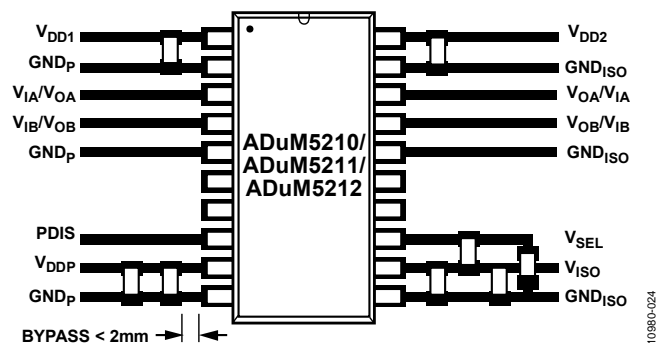
Figure 26. Recommended PCB Layout
