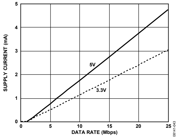
Figure 25. Typical I ISO(D) Dynamic Supply Current per Input
