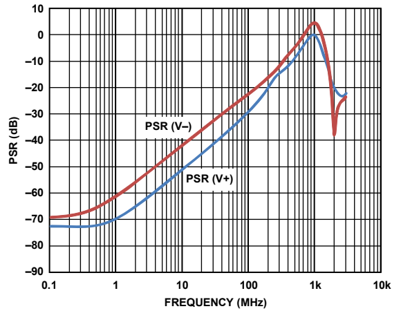
Figure 32. ADV3220 PSR
