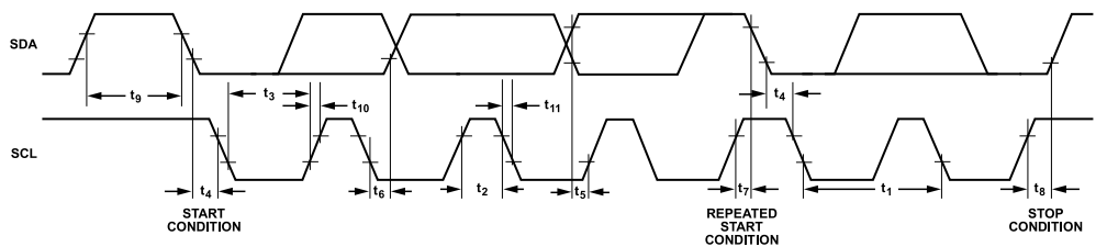
Figure 32. I 2 C Timing Diagram
