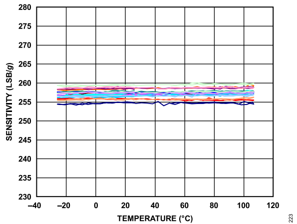
Figure 14. Y-Axis Sensitivity vs. Temperature—Eight Parts Soldered to PCB, V_S = 2.5\text{ V} , Full Resolution
