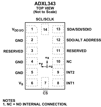
Figure 3. Pin Configuration (Top View)
