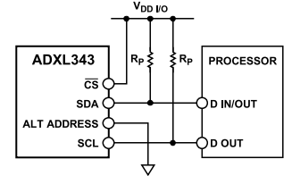
Figure 30. I 2 C Connection Diagram (Address 0x53)
