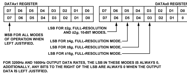
Figure 40. Data Formatting of Full-Resolution and ±2 g, 10-Bit Modes of Operation When Output Data Is Left Justified
