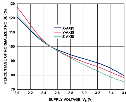
Figure 43. Normalized Noise vs. Supply Voltage, V_S
