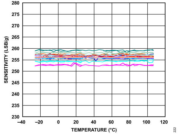
Figure 13. X-Axis Sensitivity vs. Temperature—Eight Parts Soldered to PCB, V_S = 2.5\text{ V} , Full Resolution
