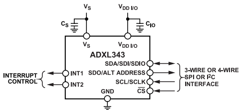
Figure 34. Application Diagram
