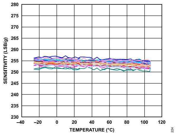
Figure 15. Z-Axis Sensitivity vs. Temperature—Eight Parts Soldered to PCB, V_S = 2.5\text{ V} , Full Resolution
