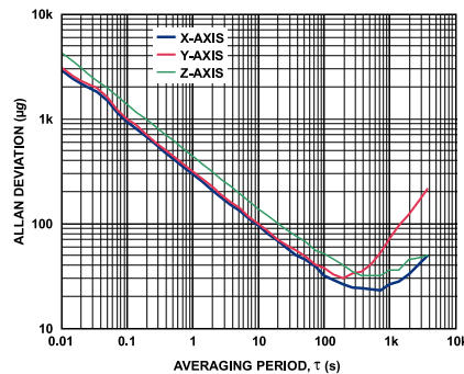
Figure 42. Root Allan Deviation
